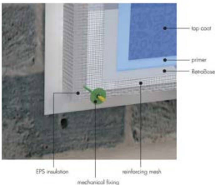
Figure 1.6 SPS Enviowall
