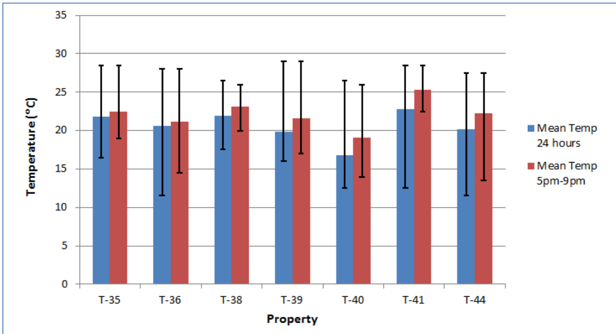
Figure 3.24 Mean living room temp for households at Ashfield Park after JUB Jubizol installations (1 st Oct 16 to 31 st Mar 17) The errors bars show the range of the maximum and minimum temperatures during the period
