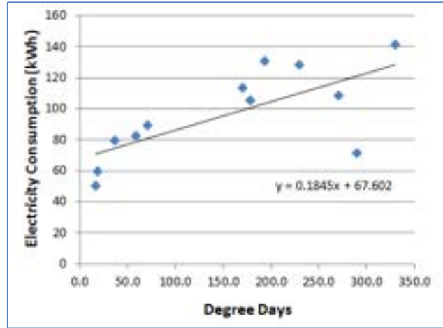
Figure 3.14b T-07 after SPS Envirowall & UF installation
