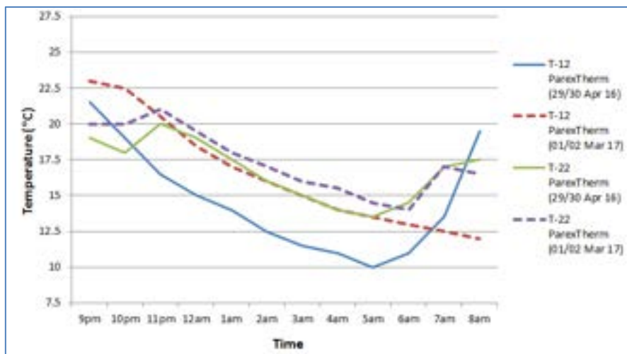
Figure 3.29b Decrease in temperature overnight before and after insulation of EWI for households T-12 and T-22 with ParexTherm Pre-installation period 29 th April 2016 (10.3 degree days) and 30 th April 2016 (8.7 degree days) Post-installation period 1 st March 2017 (10.3 degree days) and 2 nd March 2017 (9.4 degree days)
