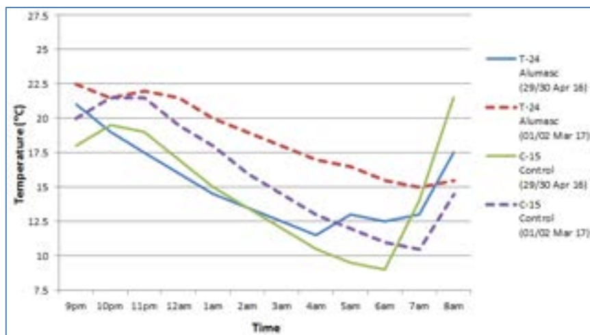
Figure 3.29c Decrease in temperature overnight for T-24 with Alumasc Swisslab EWI and C-15 the control household Pre-installation period 29 th April 2016 (10.3 degree days) and 30 th April 2016 (8.7 degree days) Post-installation period 1 st March 2017 (10.3 degree days) and 2 nd March 2017 (9.4 degree days)
