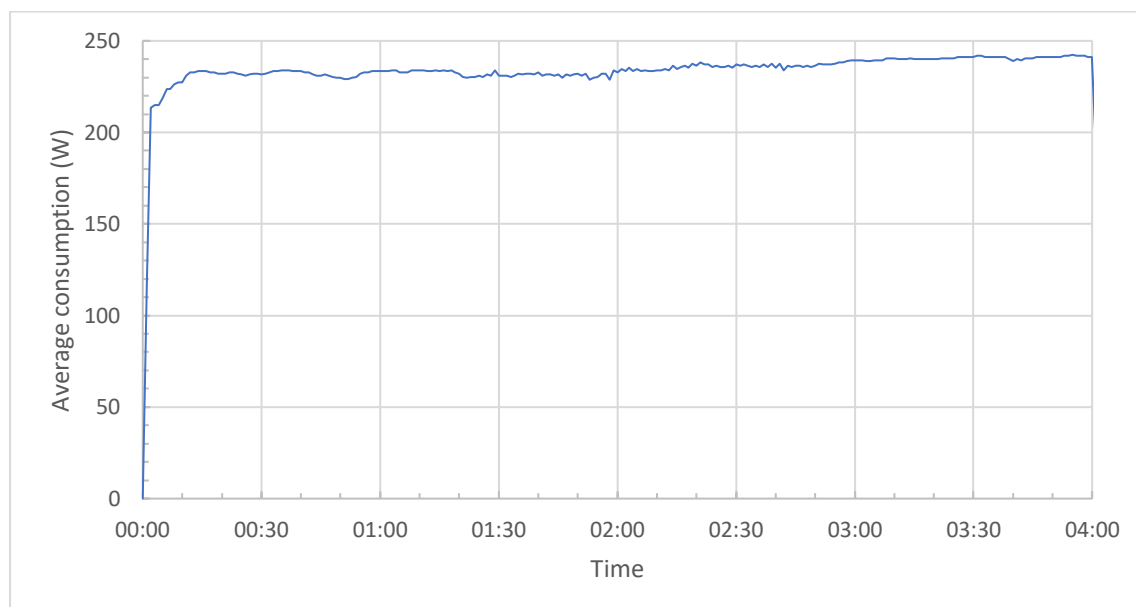
Figure 2.34 Plot of average consumption per minute measured with the Shelly Plus smart plug for the MeacoDry Arete One 20L dehumidifier and air purifier operating in a damp room Argos MDT-10DMD3
