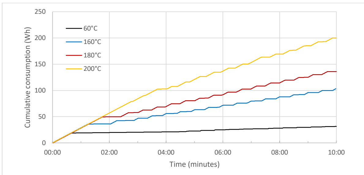
Figure 2.70 Plot of cumulative electricity consumption for the Ninja AF160 air fryer at cooking temperatures of 60°C, 160°C, 180°C and 200°C
