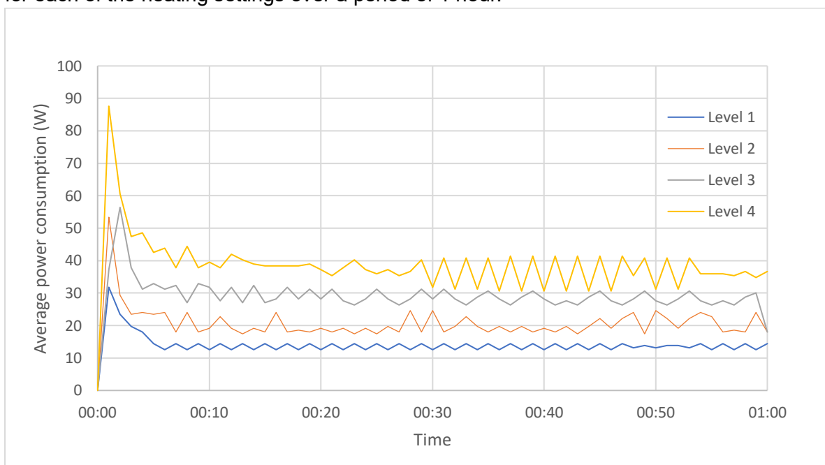
Figure 2.124 Plot of average consumption per minute measured with a Shelly Plus smart plug for the Homeglow B-warm heated seat cover on the 4 heating settings
