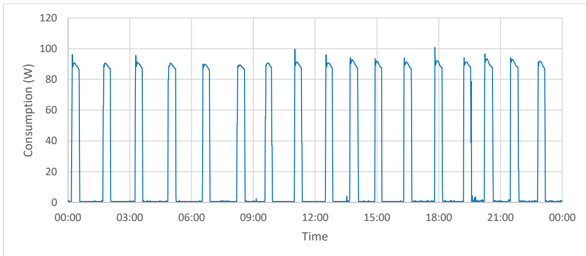
Figure 2.41 Plot of average consumption per minute measured with a Shelly Plus smart plug for the Beko K54299H/B725U fridge-freezer on 8 Feb 2024
