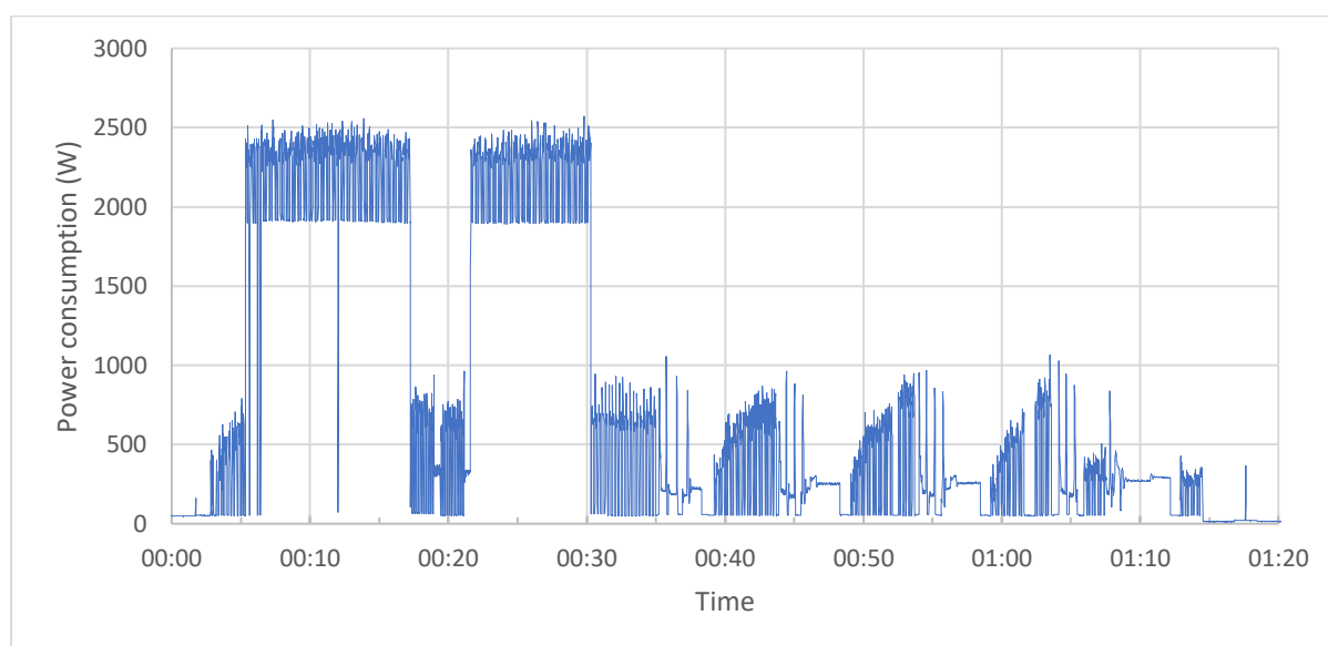
Figure 2.6 Plot of consumption for a Hotpoint WMTL80 washing machine recorded using a Tinytag View 2 data logger at 1 second intervals for a 40°C washing cycle
