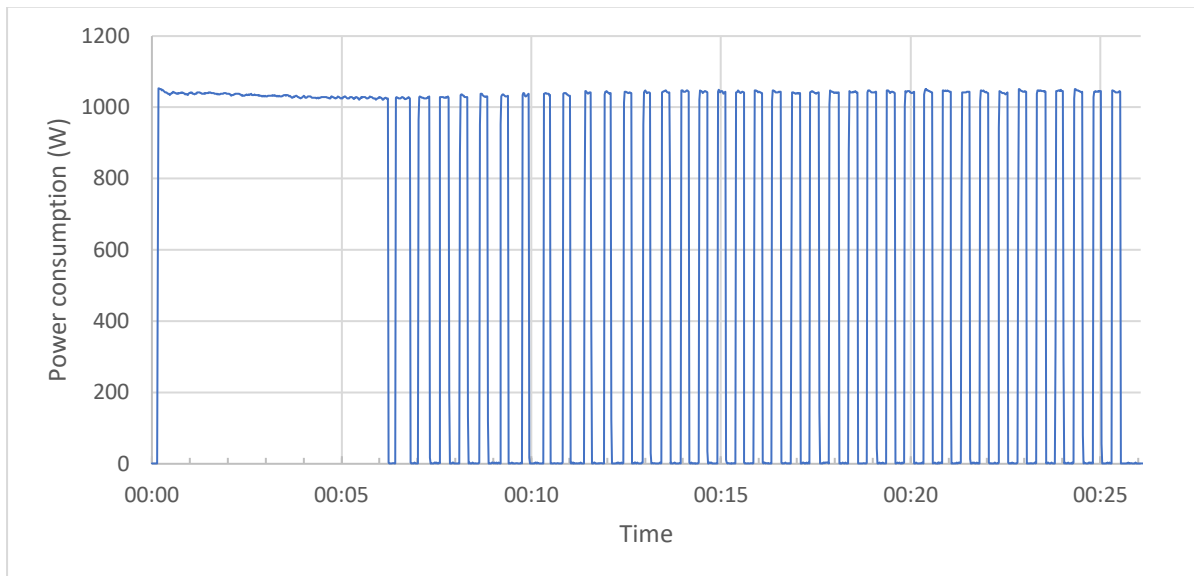
Figure 2.99 Plot of apparent power consumption measured every second with a Tinytag View 2 for the SQ Professional single electric hot plate hob on setting 5
