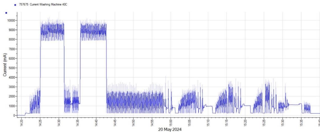
Figure 1.11 Electricity consumption of a Hotpoint WMTL80 washing machine with a 40°C wash cycle
