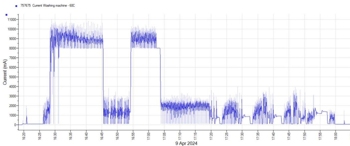
Figure 3.4 Plot of consumption for a Hotpoint WMTL80 washing machine recorded using a Tinytag View 2 data logger at 1 second intervals for a 60°C washing cycle
