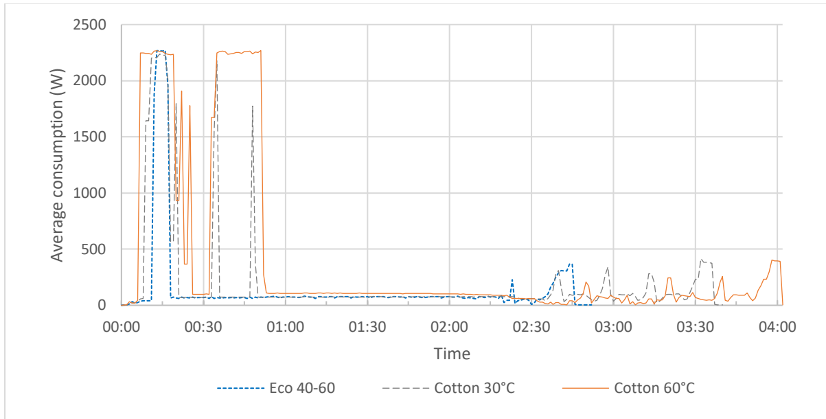
Figure 2.12 Plot of average consumption per minute measured with the Shelly Plus smart plug for the Bosch WGG04409GB on Eco 40-60 and Cotton cycles
